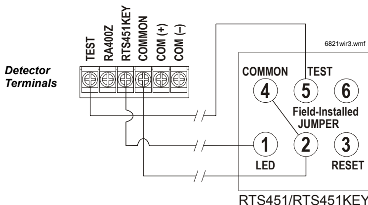
TC806D1049(CDN) Duct Smoke Detector with RTS451(A)/RTS451KEY(A).
