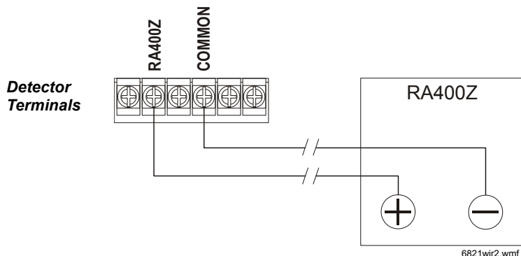
TC806D1049(CDN) Duct Smoke Detector with an optional RA400Z(A).
