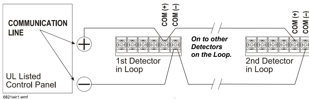
TC806D1049(CDN) Duct Smoke Detector using a UL or ULC Listed control panel.
